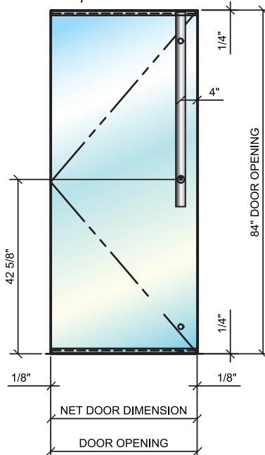
Bolt down one point lock
