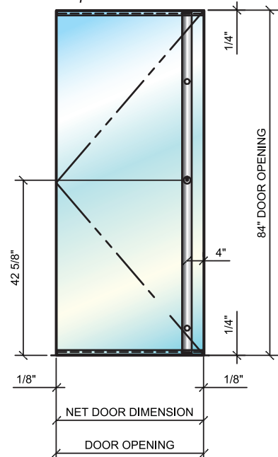
Bolt up and down two points lock
