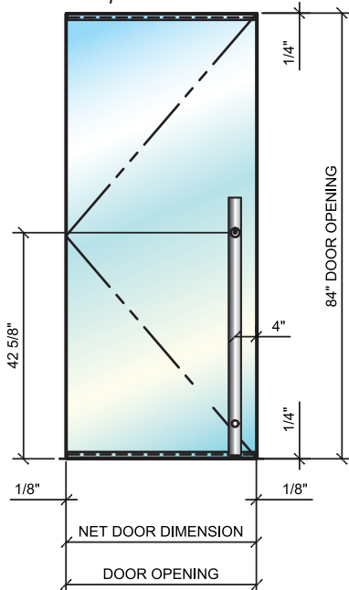
Bolt up one point lock
