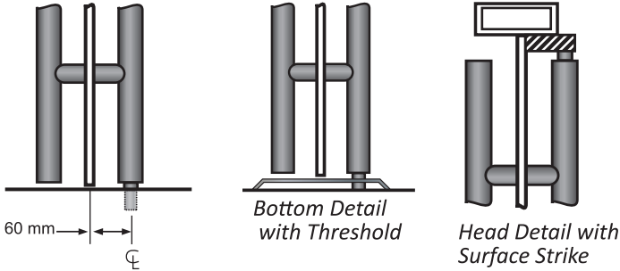
Bolt Projection Face of Door to Centerline of Bolt
